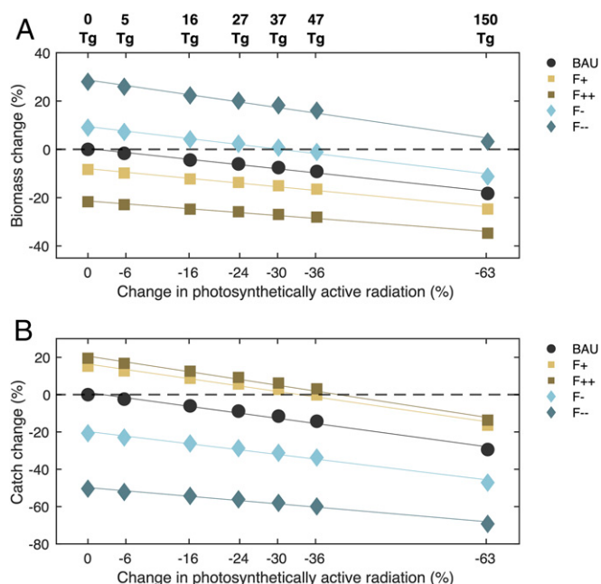
Fig. 2. Short-term impacts of nuclear war on global fisheries. Panels show the average percent difference in (A) biomass and (B) catch between the business-as-usual (BAU) control simulation (no war) and different nuclear war simulations (5 to 150 Tg), in year 2 postconflict. Each value is plotted against the war scenario (soot input indicated on upper x axis) and its associated percent reduction in global photosynthetically active radiation (PAR). The slope for each marker type shows the impact of the climatic perturbation (for a given socioeconomic response F+/-; see Table 1), while the vertical spread between marker types shows the effect of the socioeconomic responses. Statistics for linear regressions are given in SI Appendix, Tables S1 and S2 .
