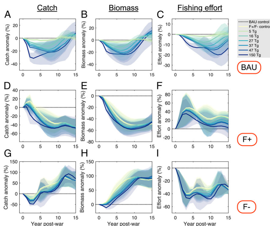
Fig. 3. Global fishery developments postwar. Panels show the percent anomaly from the BAU control scenario (dashed line) for all soot inputs (solid lines). Upper row (A–C) shows trajectories of catch, biomass, and fishing effort under BAU fishing, middle row (D–F) shows trajectories under the intensified fishing scenario F+, and lower row (G–I) shows trajectories under the decreased fishing scenarios F–. The shaded areas show SD for the five parameter ensemble runs, while the solid lines are the ensemble mean. The light yellow lines in D–I show the F+ and F– responses in the absence of a climatic perturbation, i.e., the F+ or F– control.
